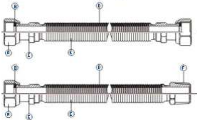
GAS Stainless Steel Corrugated Hose
